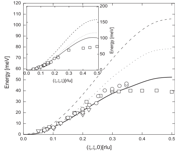
Fig. 2. Magnon dispersion along the (\xi, \xi, 0) - [(\xi, \xi, \xi)] -direction [inset]. Line styles are the same as in Fig. 1. Experimental data in main figure is taken from [1]. The Pr-(Nd-, La-) data shown in the inset is taken from [3] ([2]).
