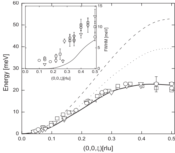
Fig. 1. Magnon dispersion along the (0,0,\xi) -direction. The dashed line corresponds to the function \omega_p . The solid (dotted) line gives \tilde{\omega}_p with (without) contribution from the orbital collective mode. Inset: Magnon width 2\tilde{\Gamma}_p . Here squares, triangles and circles give experimental data [1] for \text{Pr}_{0.63}\text{Sr}_{0.37}\text{MnO}_3 , \text{Nd}_{0.7}\text{Sr}_{0.3}\text{MnO}_3 , and \text{La}_{0.7}\text{Ca}_{0.3}\text{MnO}_3 , respectively.
